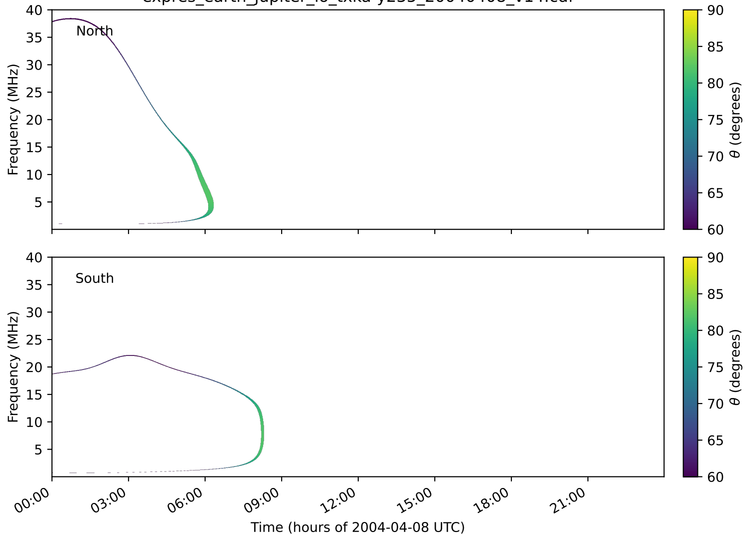
expres_earth_jupiter_io_txka-y235_20040408_v14.cdf
