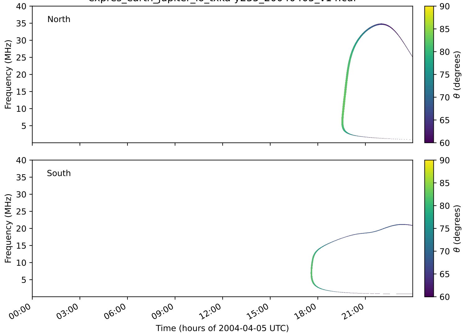
expres_earth_jupiter_io_txka-y235_20040405_v14.cdf
