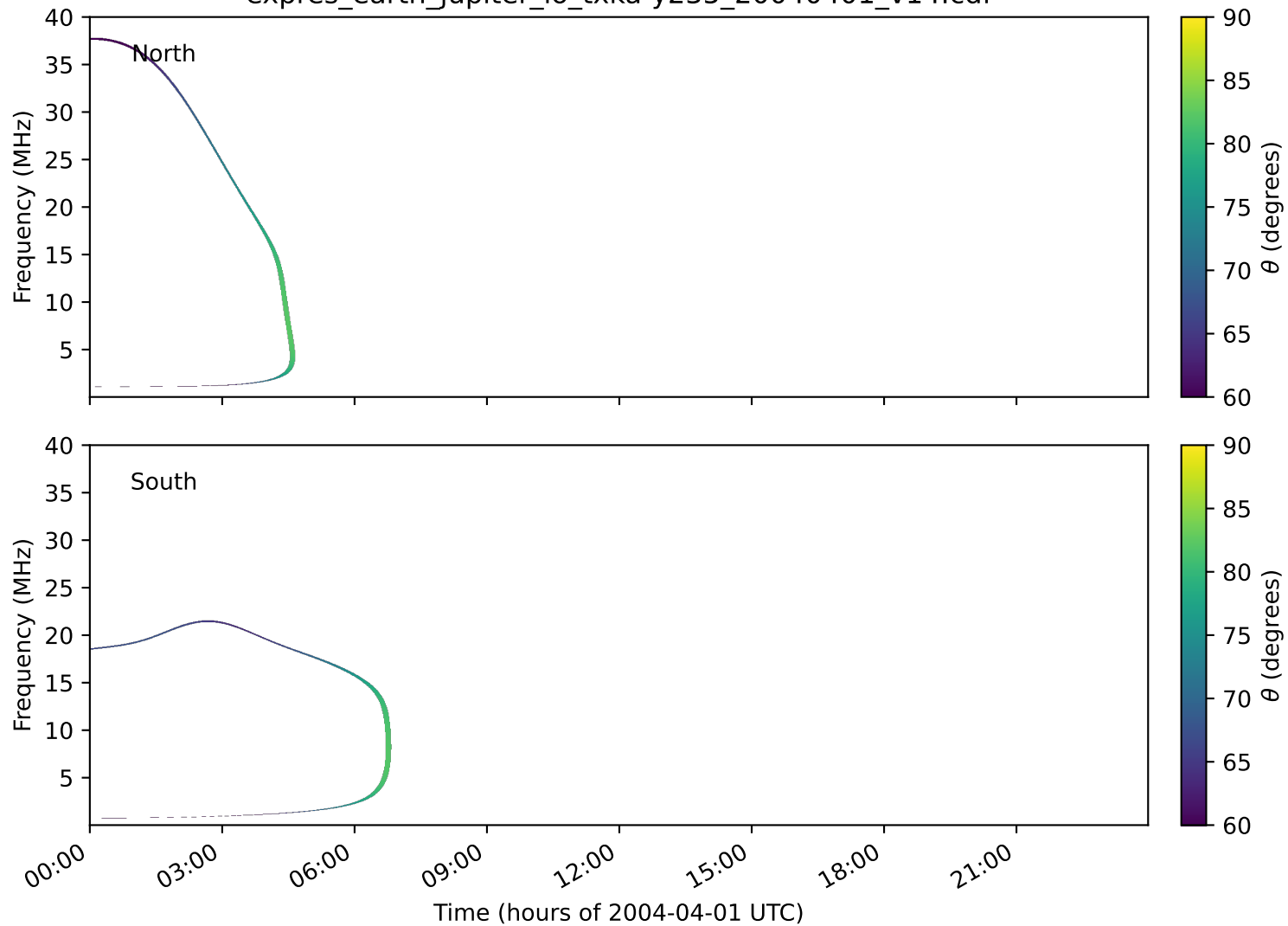
expres_earth_jupiter_io_txka-y235_20040401_v14.cdf
