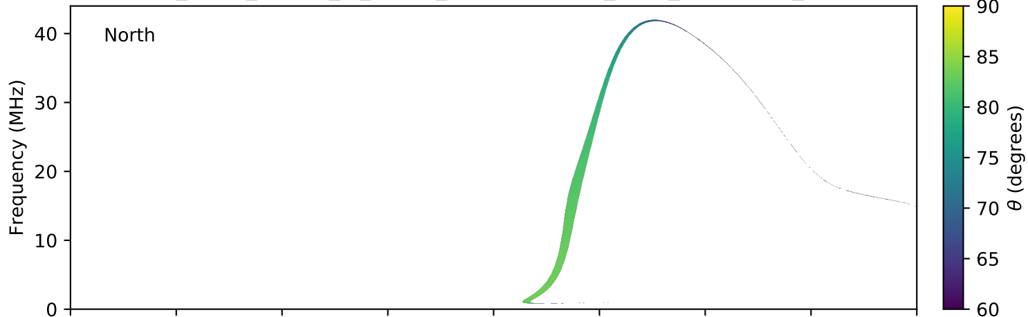
expres_earth_jupiter_io_jrm09_lossc-wid1deg_3kev_20040430_v11.cdf
