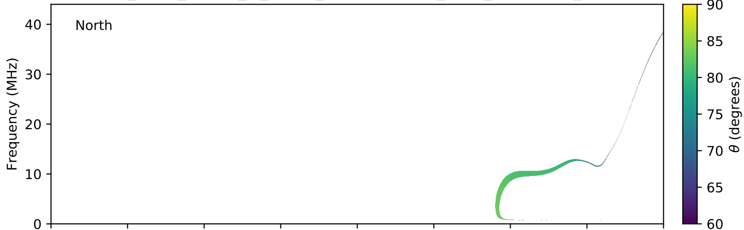
expres_earth_jupiter_io_jrm09_lossc-wid1deg_3kev_20040428_v11.cdf
