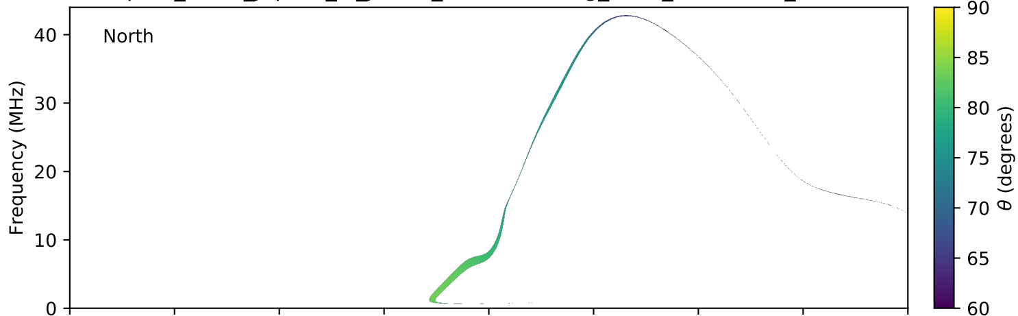
expres_earth_jupiter_io_jrm09_lossc-wid1deg_3kev_20040423_v11.cdf
