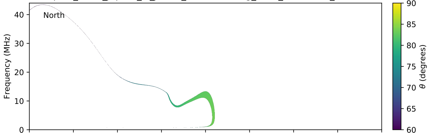
expres_earth_jupiter_io_jrm09_lossc-wid1deg_3kev_20040422_v11.cdf
