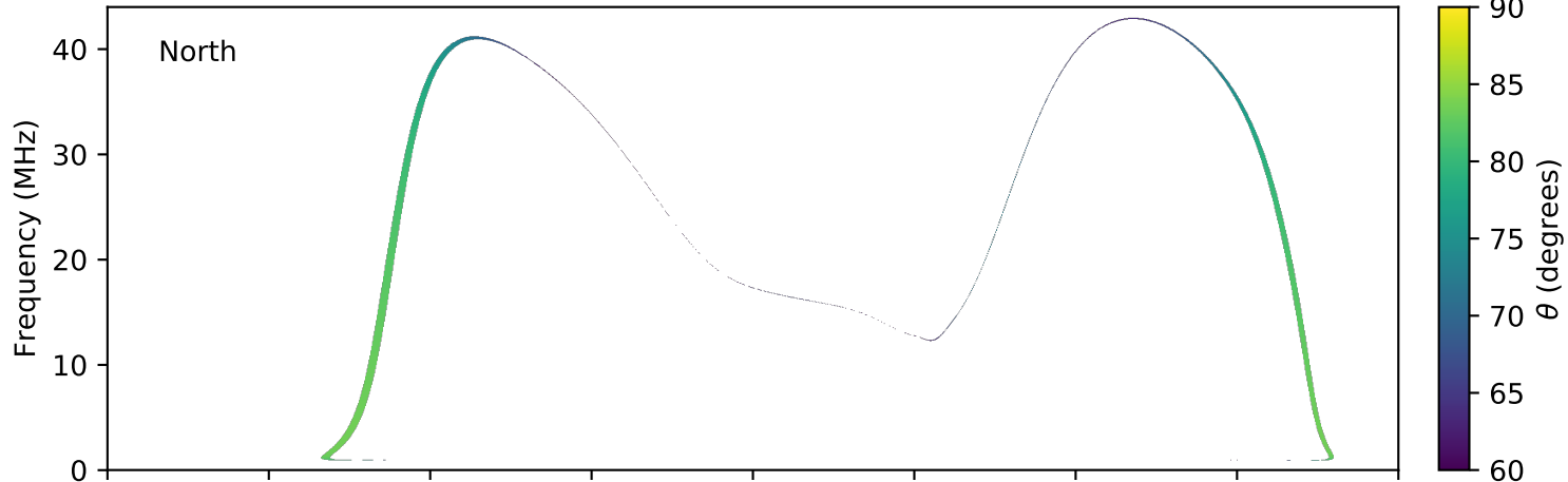
expres_earth_jupiter_io_jrm09_lossc-wid1deg_3kev_20040418_v11.cdf
