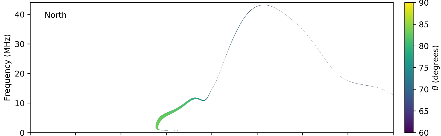
expres_earth_jupiter_io_jrm09_lossc-wid1deg_3kev_20040416_v11.cdf
