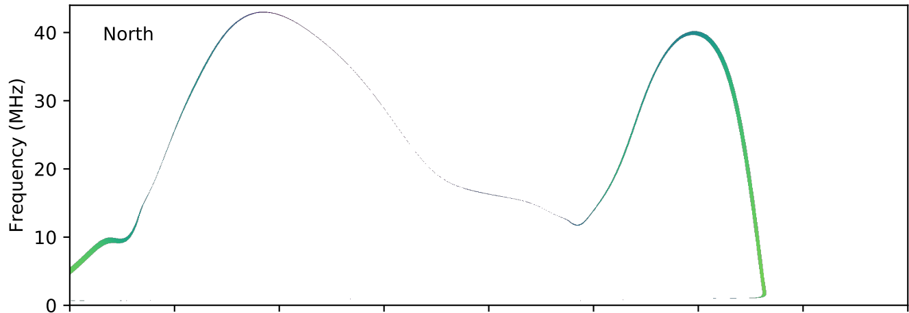
expres_earth_jupiter_io_jrm09_lossc-wid1deg_3kev_20040404_v11.cdf
