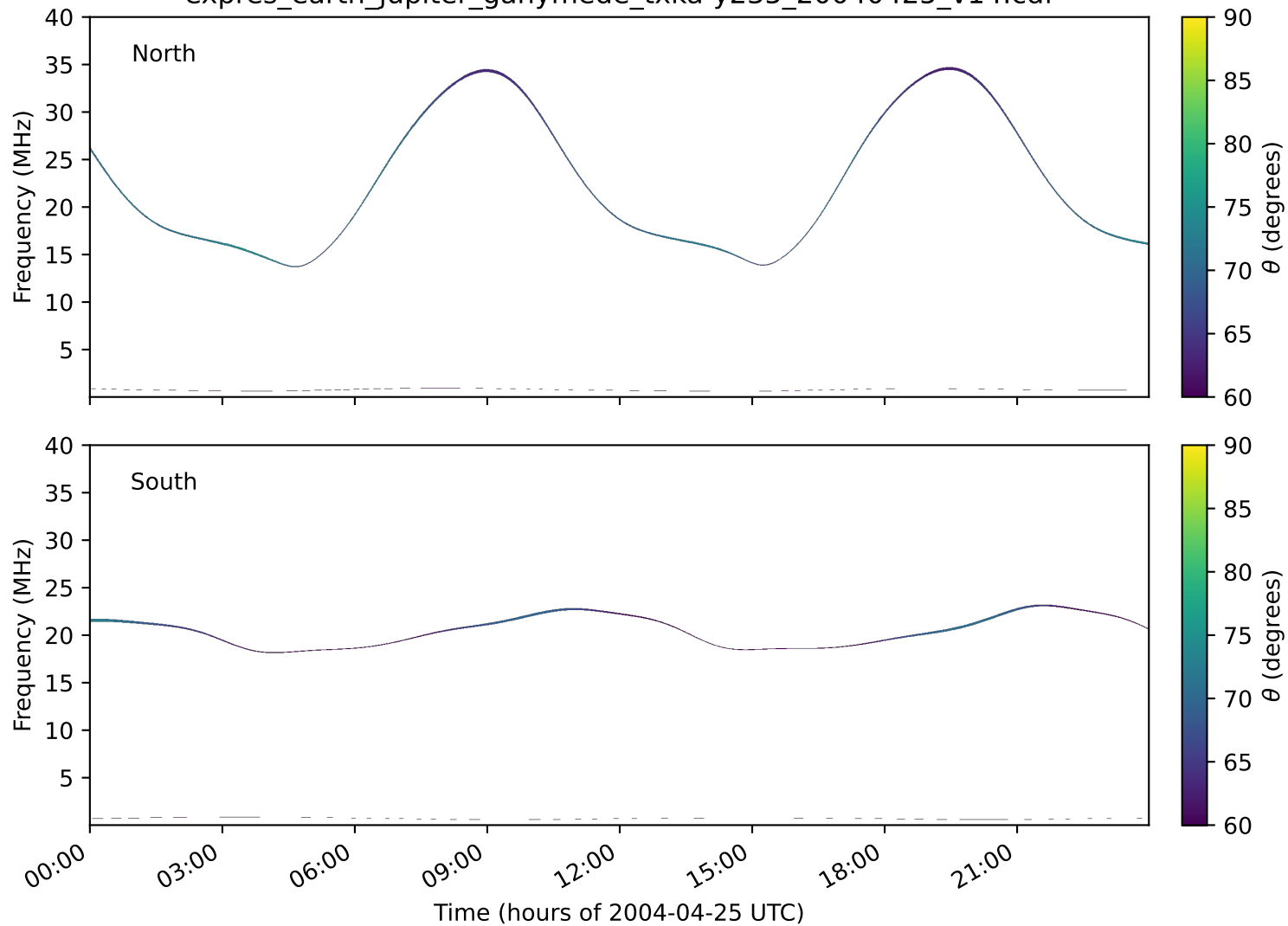
expres_earth_jupiter_ganymede_txka-y235_20040425_v14.cdf
