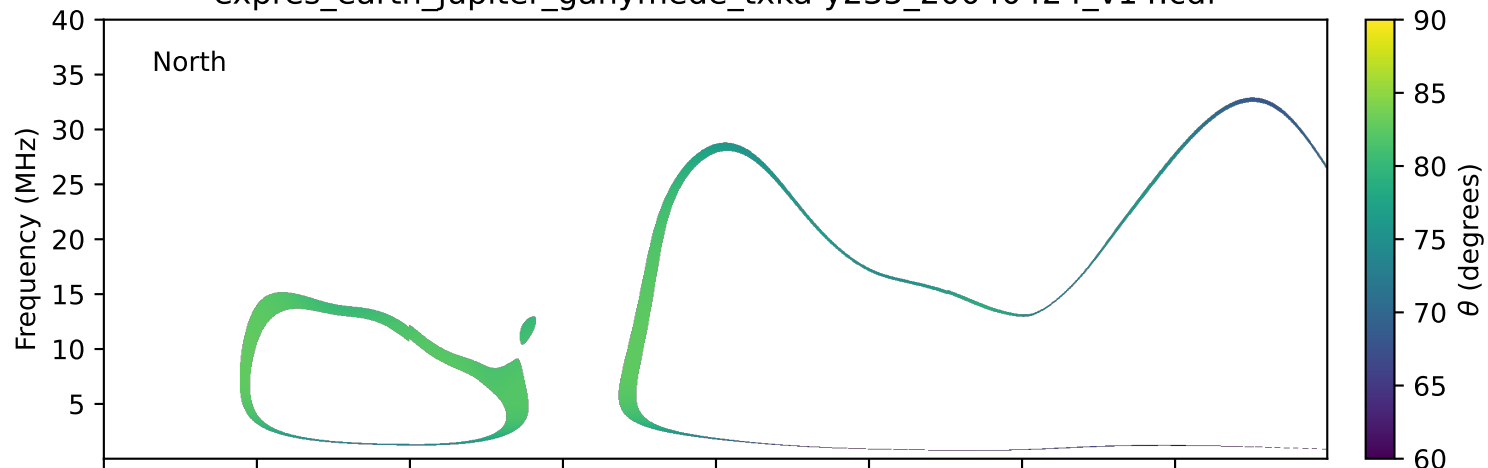
expres_earth_jupiter_ganymede_txka-y235_20040424_v14.cdf
