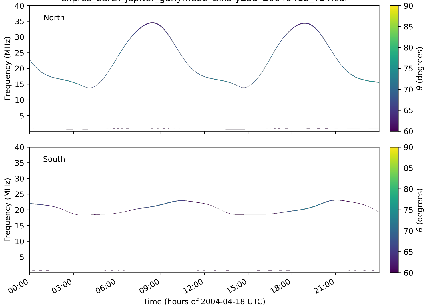
expres_earth_jupiter_ganymede_txka-y235_20040418_v14.cdf
