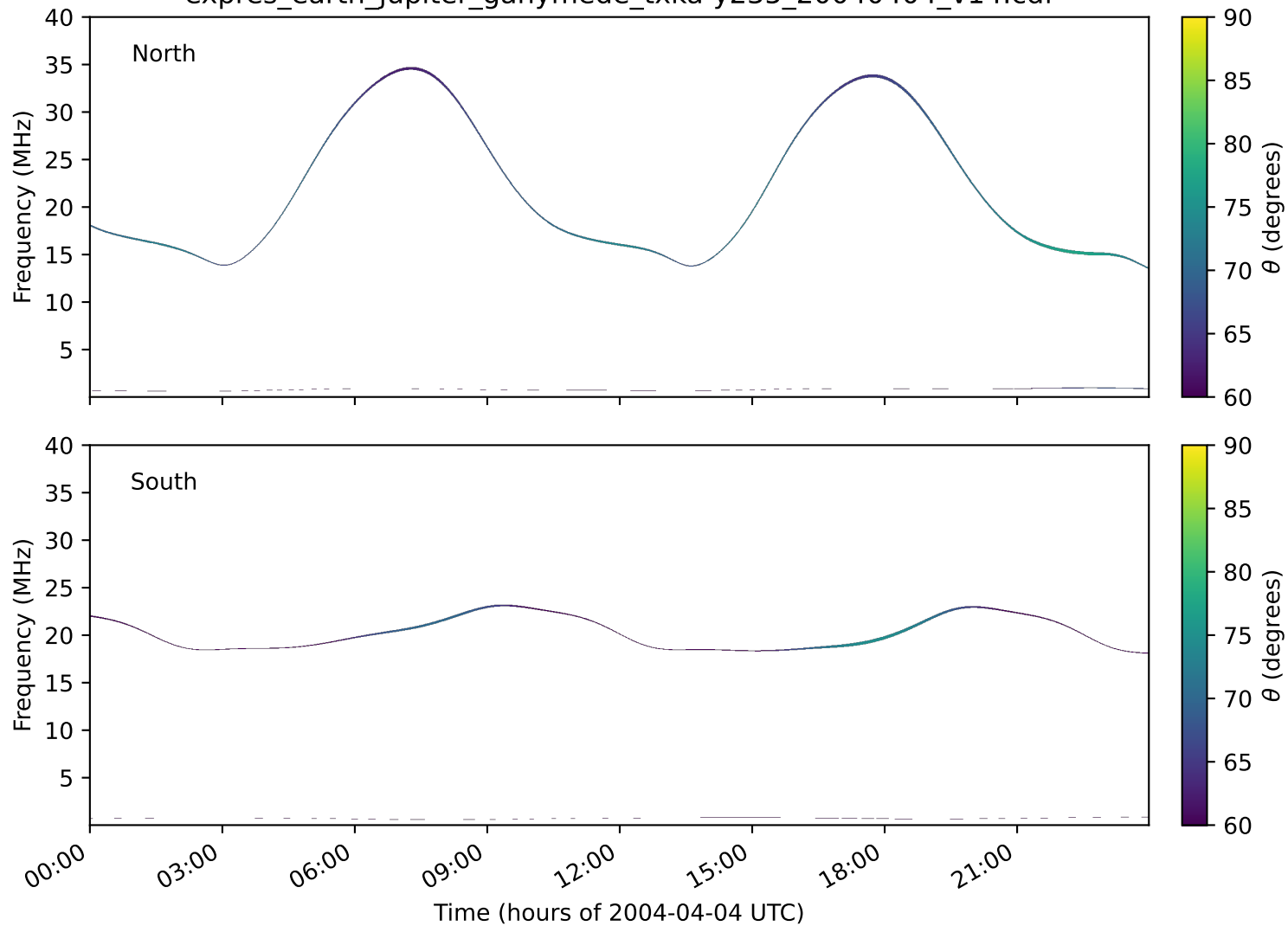
expres_earth_jupiter_ganymede_txka-y235_20040404_v14.cdf
