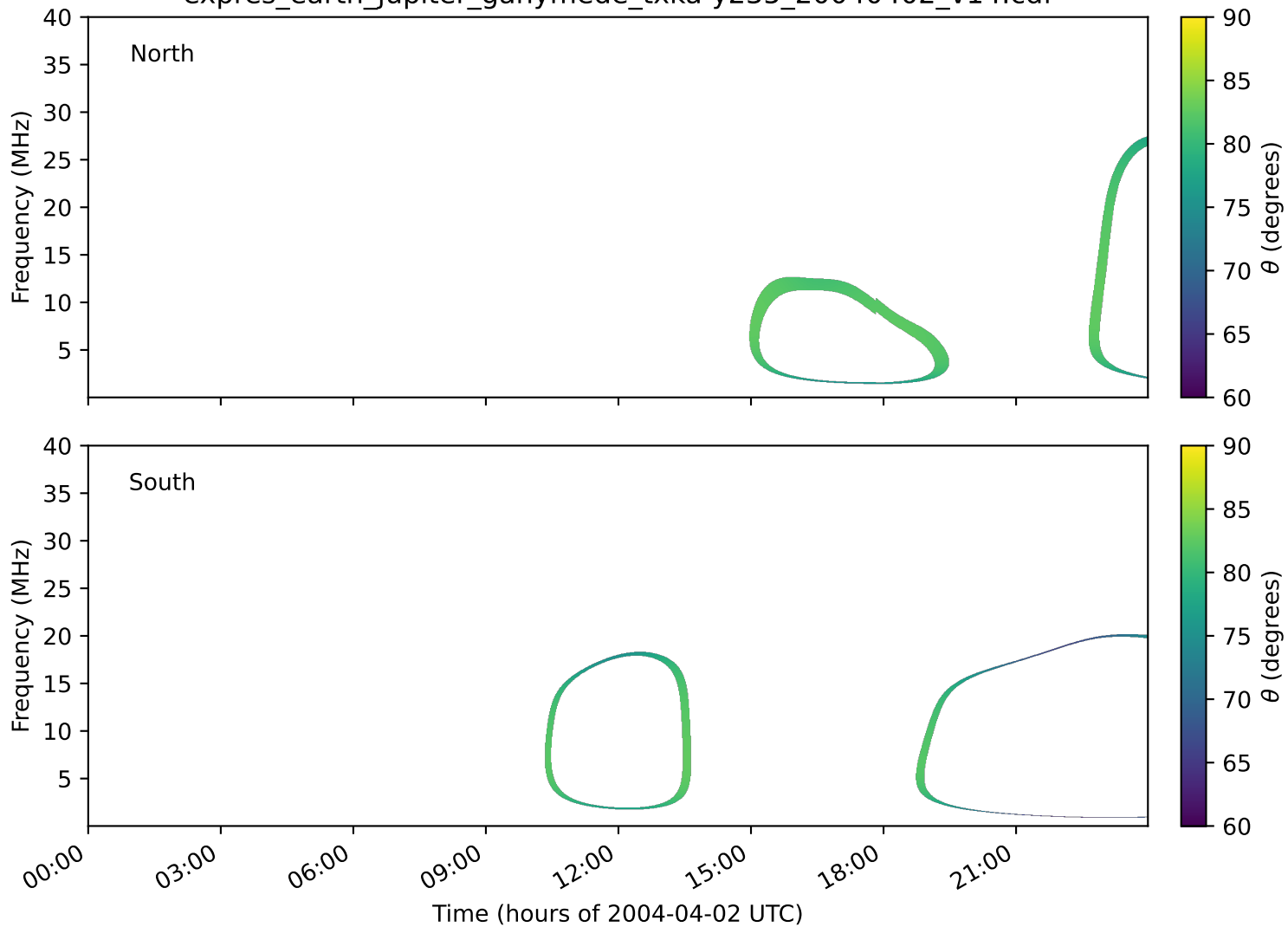
expres_earth_jupiter_ganymede_txka-y235_20040402_v14.cdf
