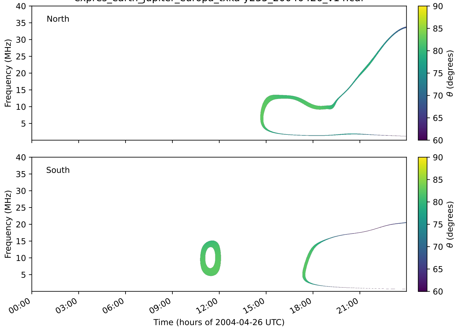
expres_earth_jupiter_europa_txka-y235_20040426_v14.cdf
