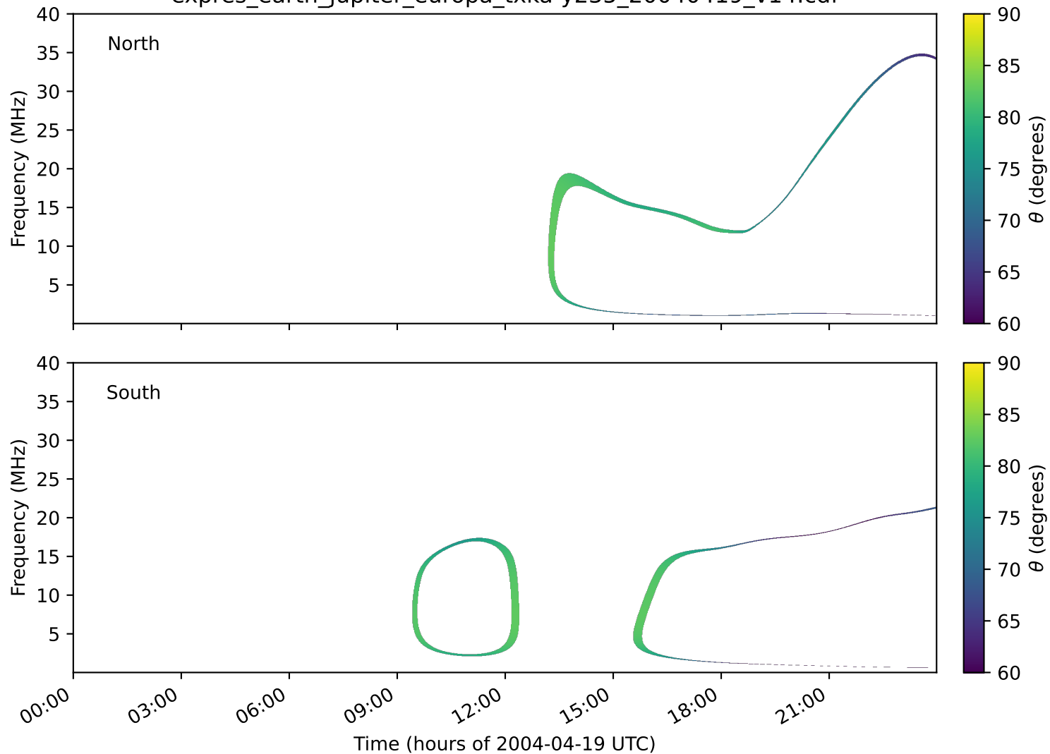
expres_earth_jupiter_europa_txka-y235_20040419_v14.cdf
