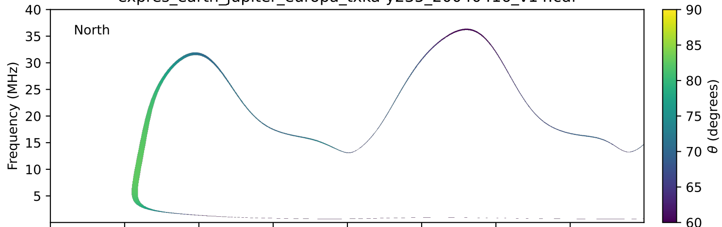
expres_earth_jupiter_europa_txka-y235_20040416_v14.cdf
