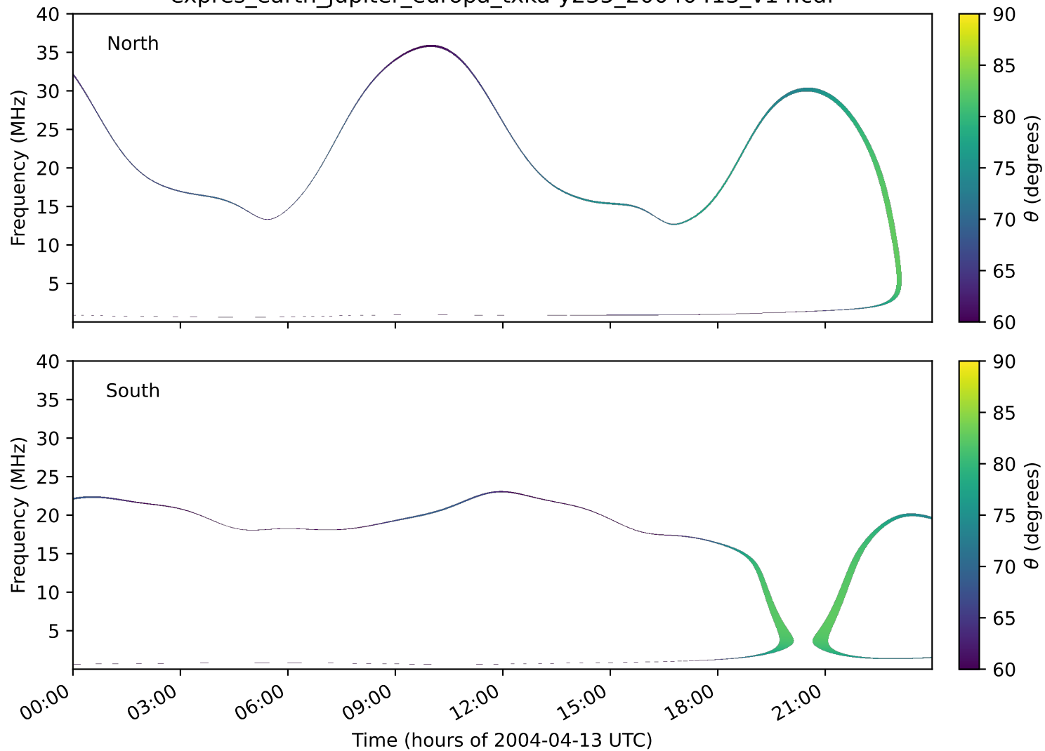
expres_earth_jupiter_europa_txka-y235_20040413_v14.cdf
