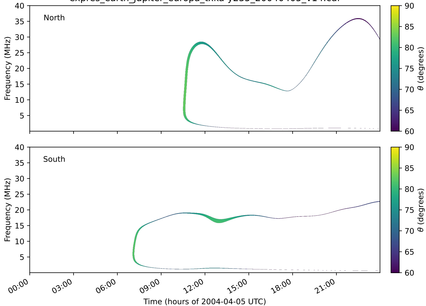
expres_earth_jupiter_europa_txka-y235_20040405_v14.cdf
