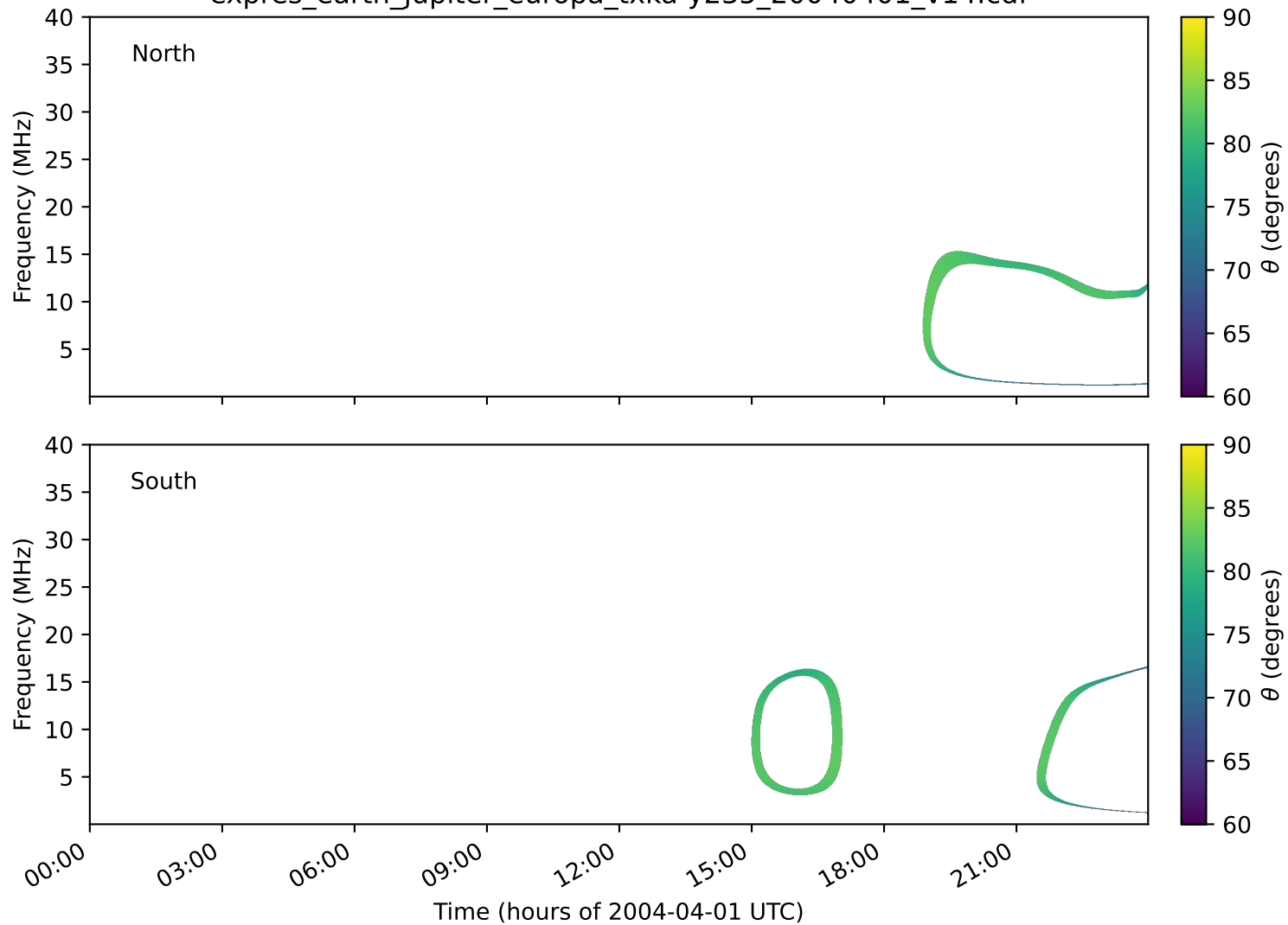
expres_earth_jupiter_europa_txka-y235_20040401_v14.cdf
