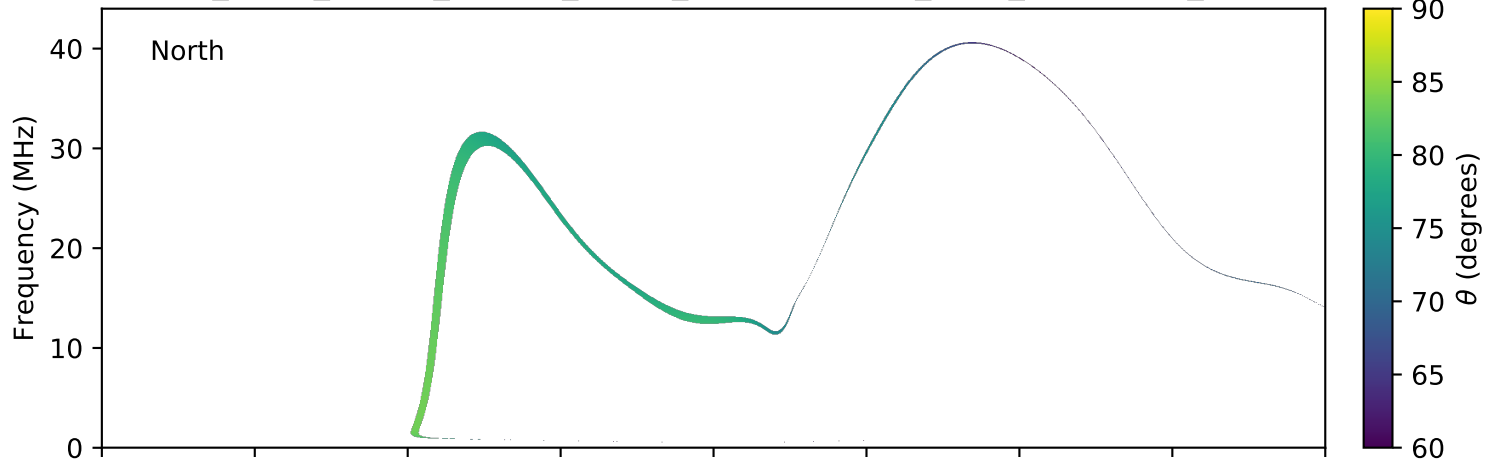
expres_earth_jupiter_europa_jrm09_lossc-wid1deg_3kev_20040430_v11.cdf
