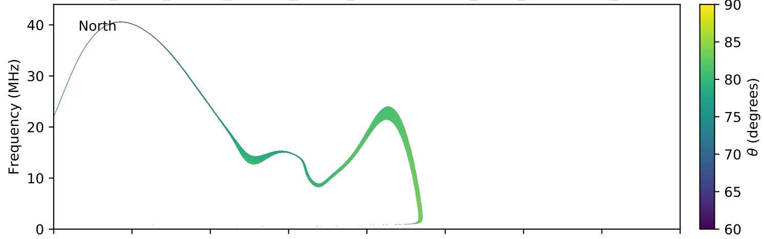
expres_earth_jupiter_europa_jrm09_lossc-wid1deg_3kev_20040410_v11.cdf
