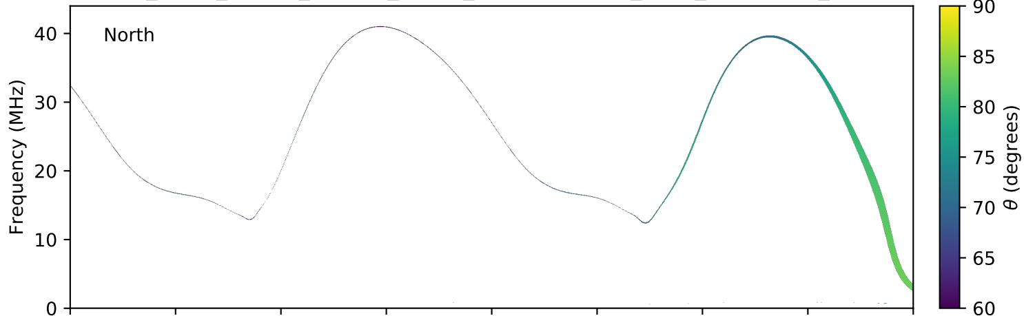
expres_earth_jupiter_europa_jrm09_lossc-wid1deg_3kev_20040406_v11.cdf
