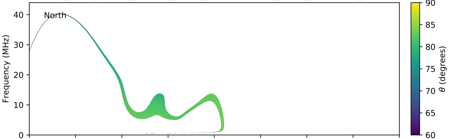
expres_earth_jupiter_europa_jrm09_lossc-wid1deg_3kev_20040403_v11.cdf
