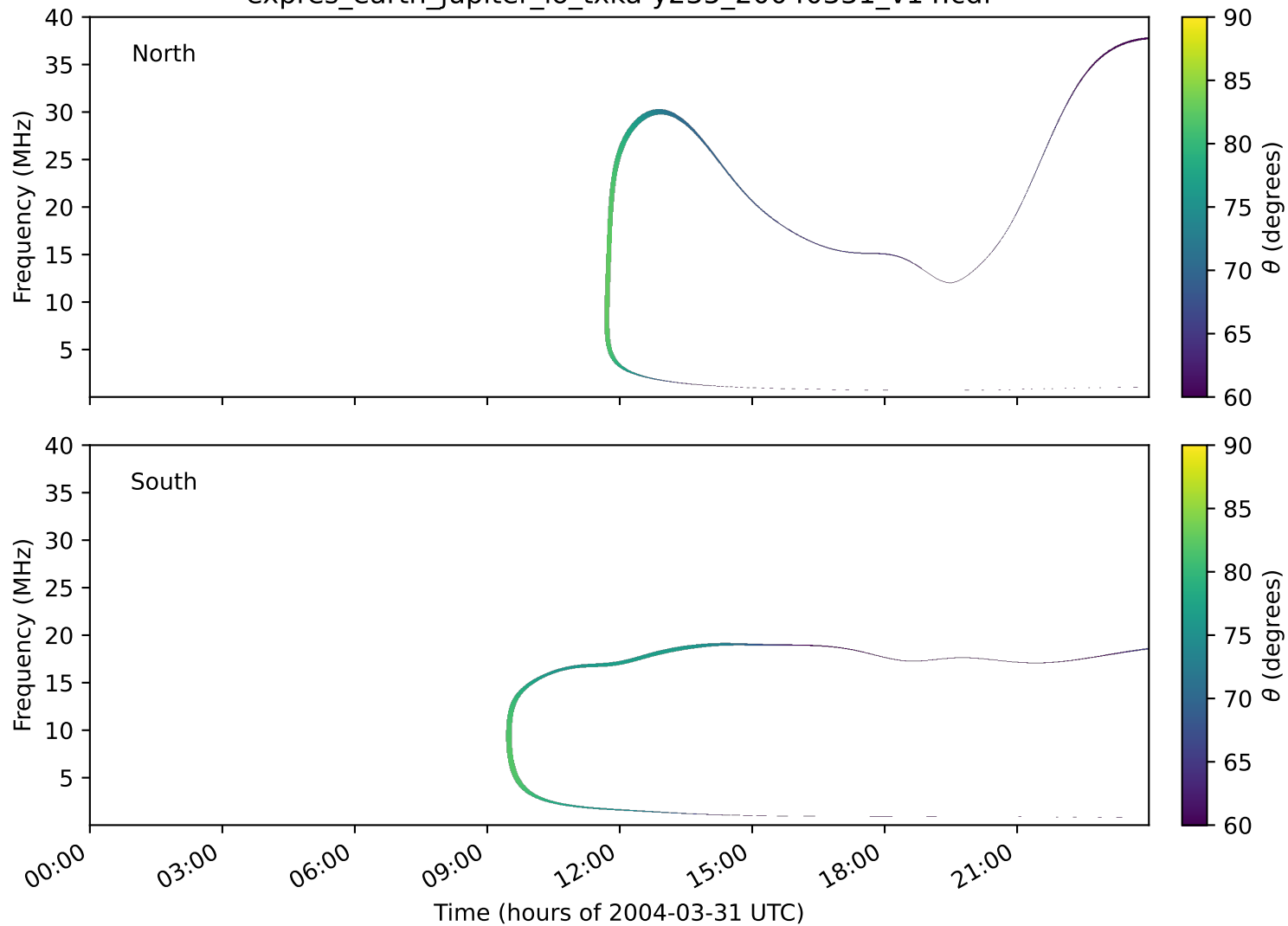
expres_earth_jupiter_io_txka-y235_20040331_v14.cdf
