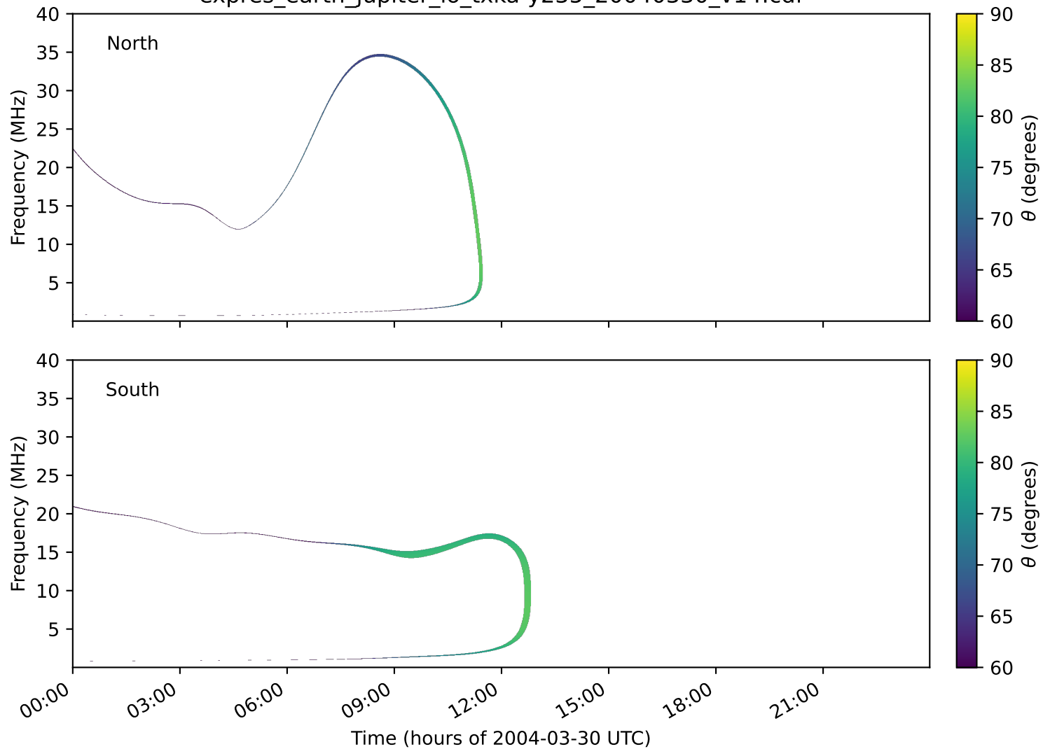
expres_earth_jupiter_io_txka-y235_20040330_v14.cdf
