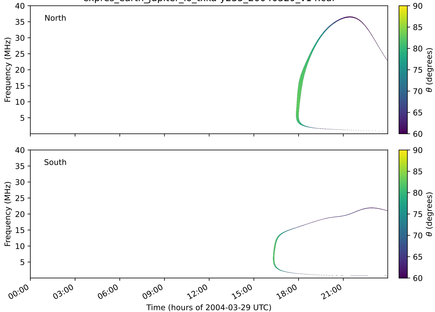
expres_earth_jupiter_io_txka-y235_20040329_v14.cdf
