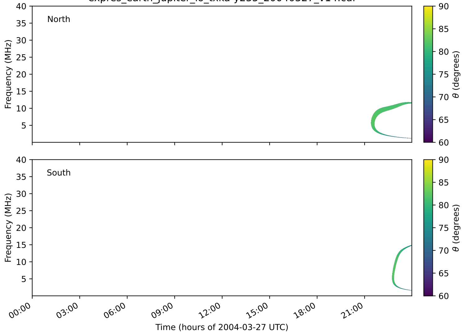
expres_earth_jupiter_io_txka-y235_20040327_v14.cdf
