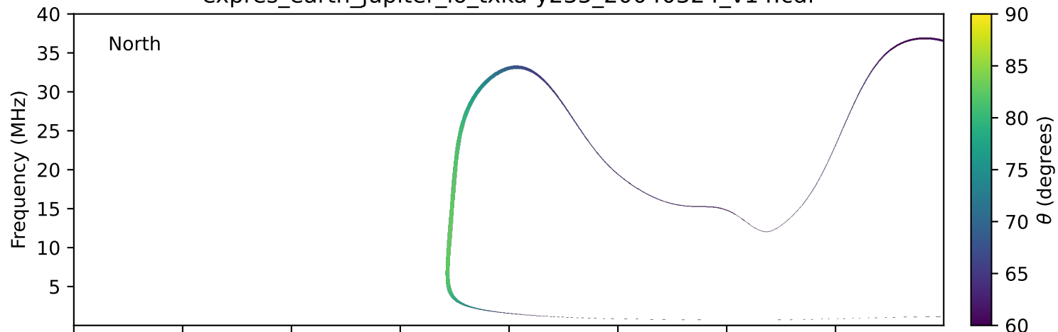
expres_earth_jupiter_io_txka-y235_20040324_v14.cdf
