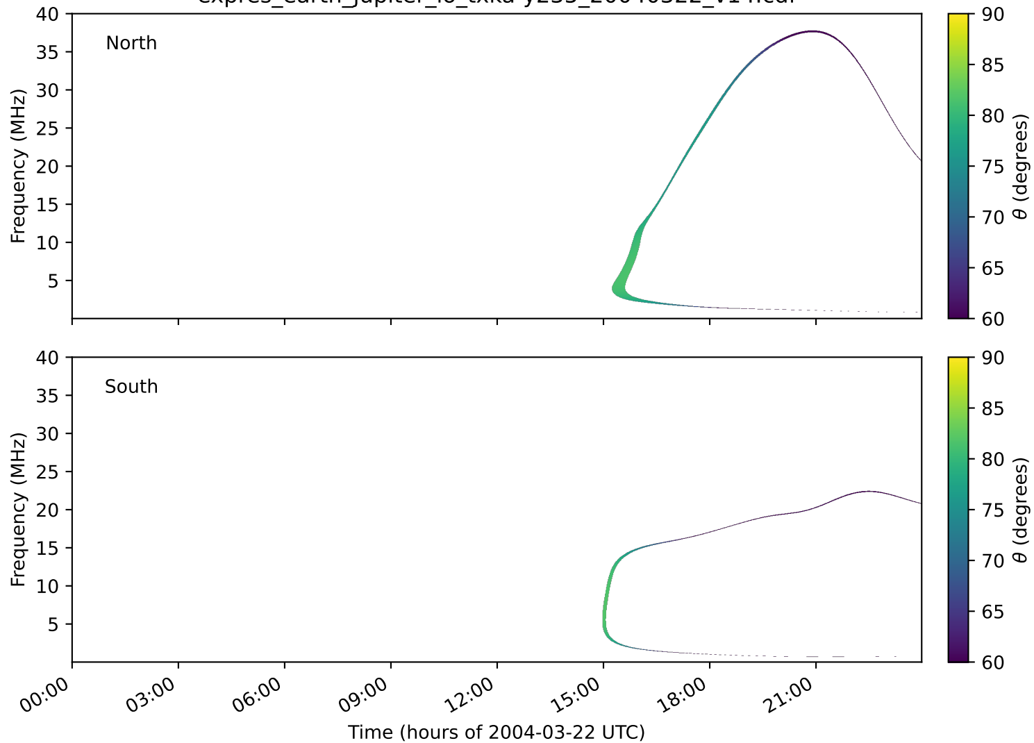
expres_earth_jupiter_io_txka-y235_20040322_v14.cdf
