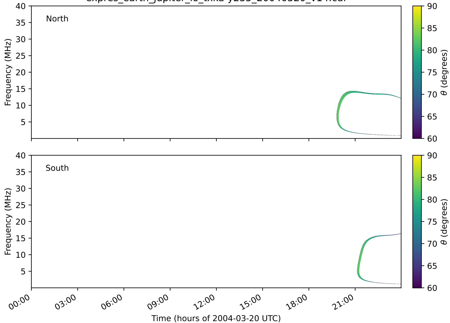
expres_earth_jupiter_io_txka-y235_20040320_v14.cdf
