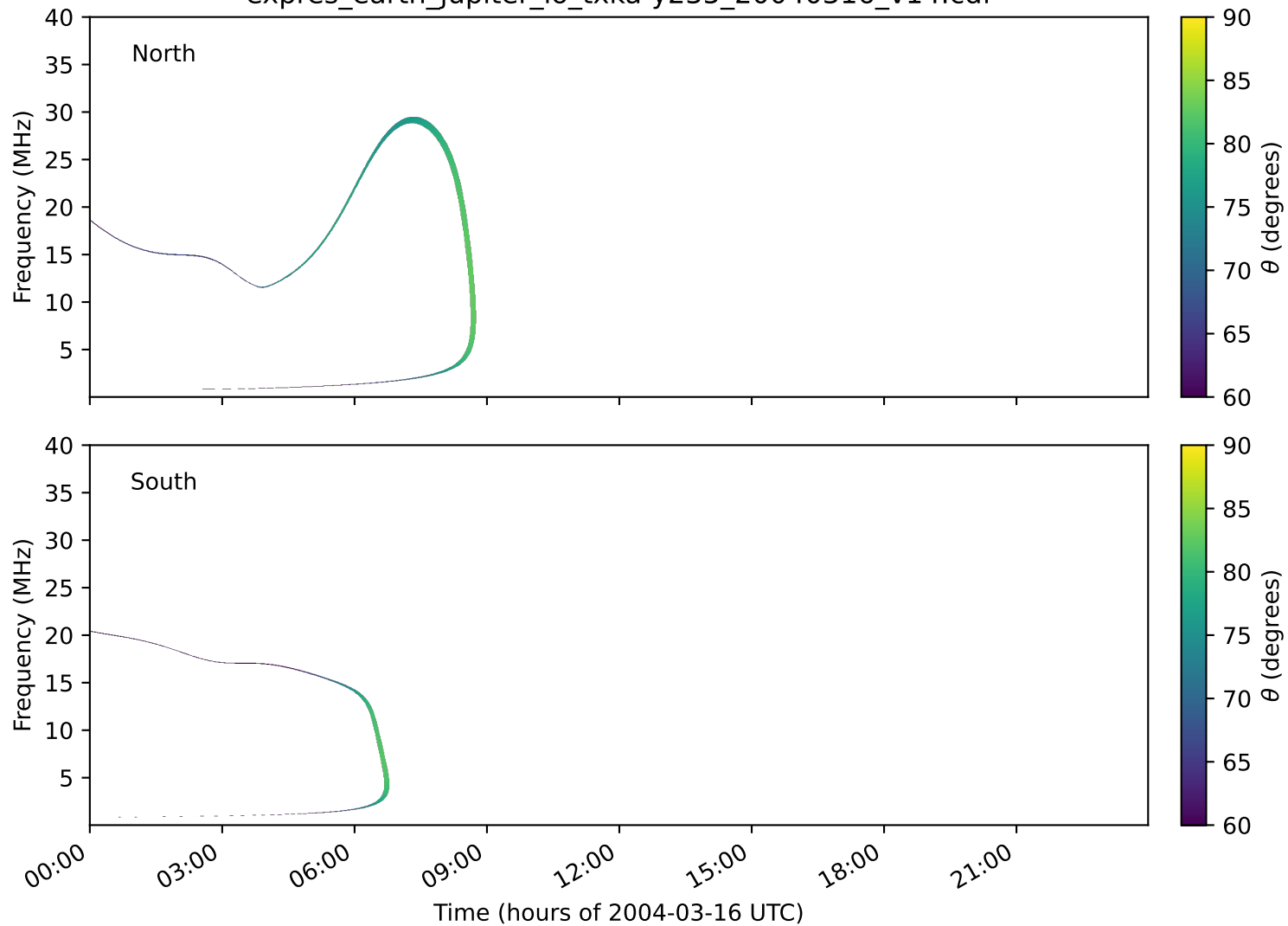
expres_earth_jupiter_io_txka-y235_20040316_v14.cdf
