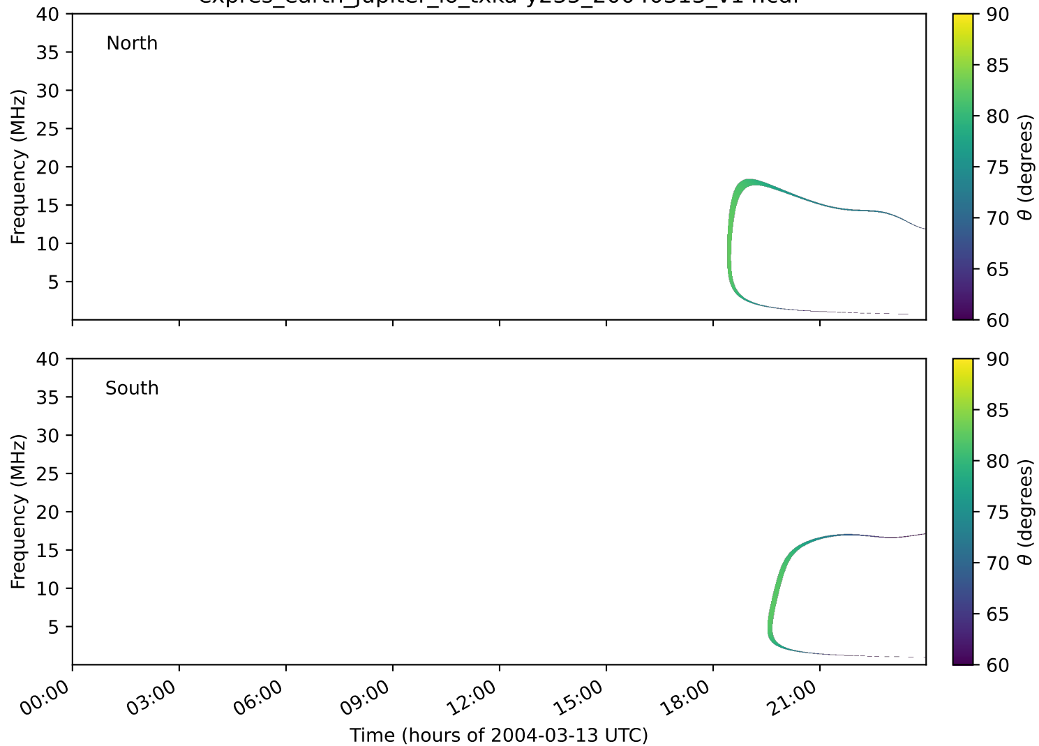
expres_earth_jupiter_io_txka-y235_20040313_v14.cdf
