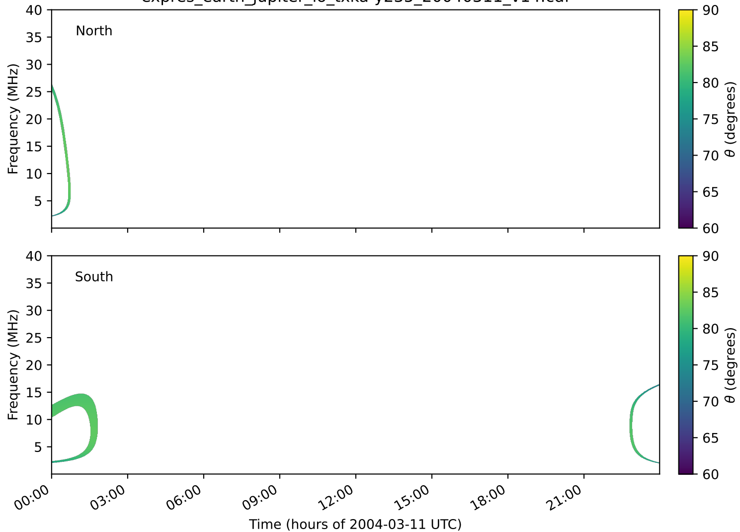
expres_earth_jupiter_io_txka-y235_20040311_v14.cdf
