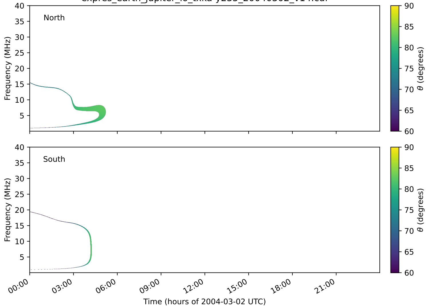
expres_earth_jupiter_io_txka-y235_20040302_v14.cdf
