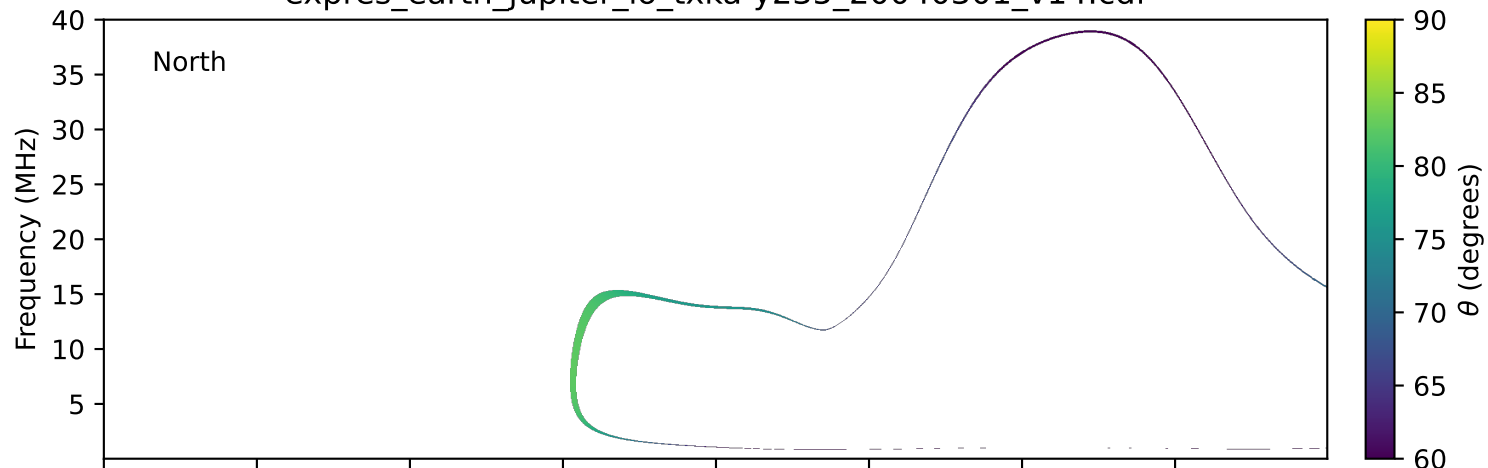
expres_earth_jupiter_io_txka-y235_20040301_v14.cdf
