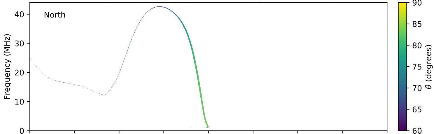
expres_earth_jupiter_io_jrm09_lossc-wid1deg_3kev_20040330_v11.cdf
