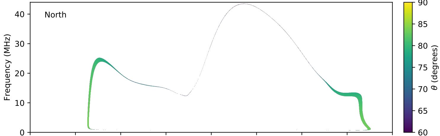
expres_earth_jupiter_io_jrm09_lossc-wid1deg_3kev_20040326_v11.cdf
