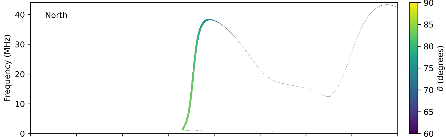
expres_earth_jupiter_io_jrm09_lossc-wid1deg_3kev_20040324_v11.cdf
