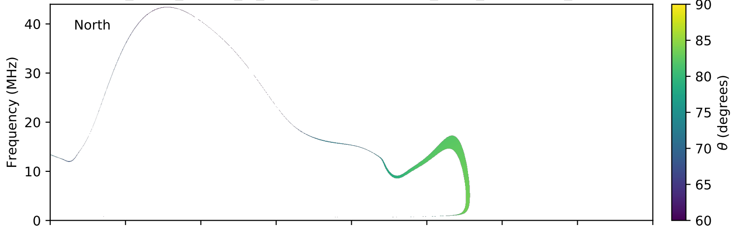
expres_earth_jupiter_io_jrm09_lossc-wid1deg_3kev_20040321_v11.cdf
