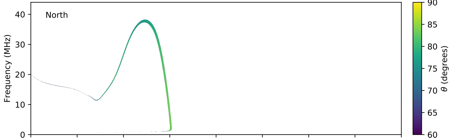
expres_earth_jupiter_io_jrm09_lossc-wid1deg_3kev_20040316_v11.cdf
