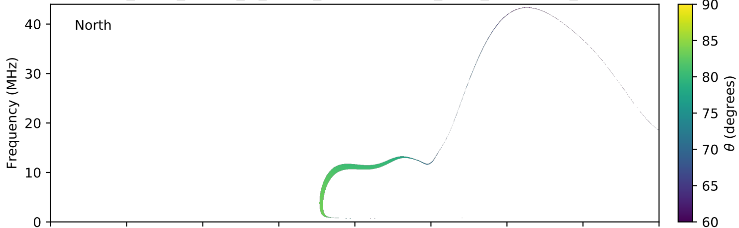
expres_earth_jupiter_io_jrm09_lossc-wid1deg_3kev_20040308_v11.cdf
