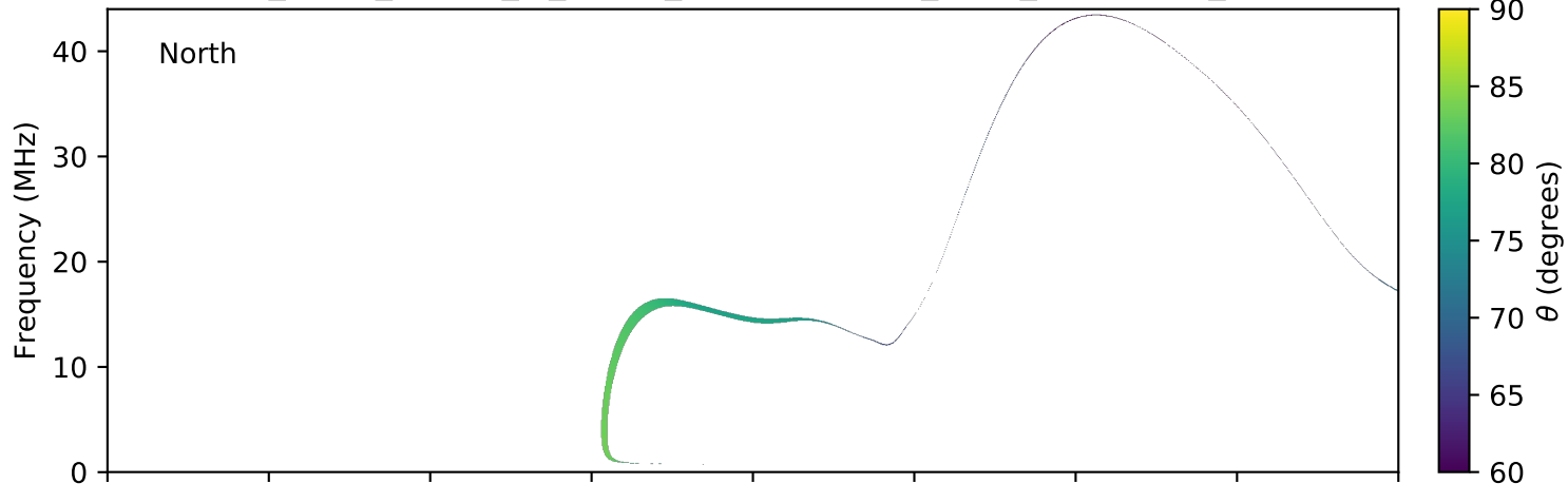
expres_earth_jupiter_io_jrm09_lossc-wid1deg_3kev_20040301_v11.cdf
