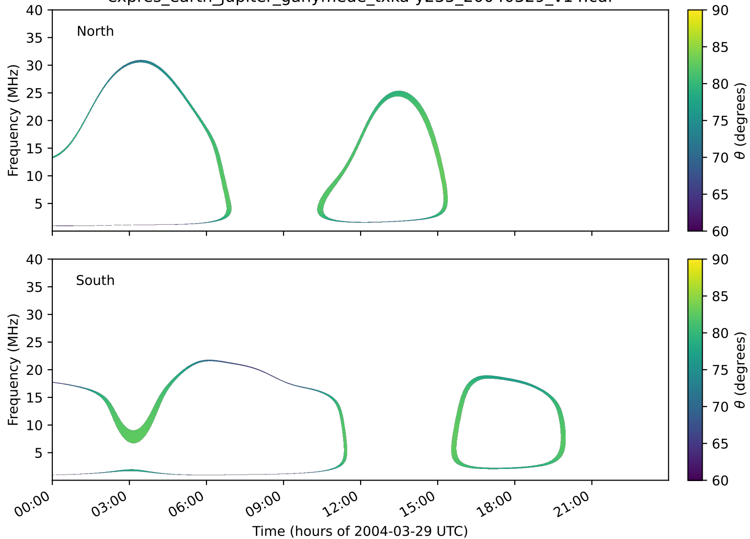
expres_earth_jupiter_ganymede_txka-y235_20040329_v14.cdf
