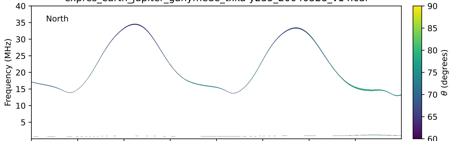
expres_earth_jupiter_ganymede_txka-y235_20040328_v14.cdf
