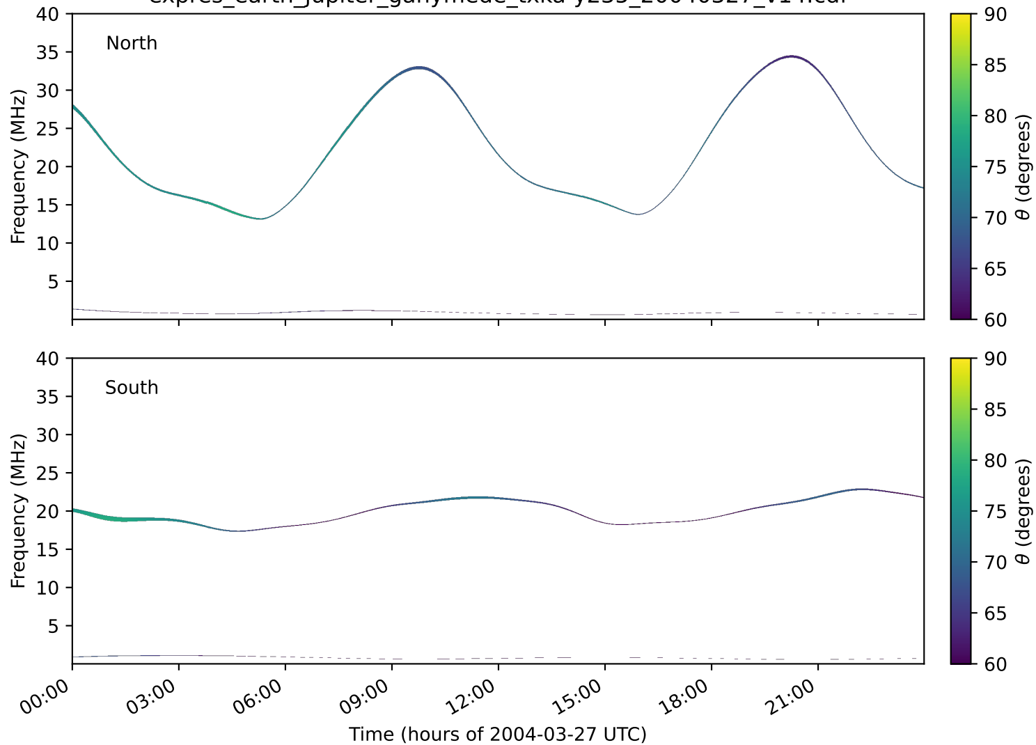
expres_earth_jupiter_ganymede_txka-y235_20040327_v14.cdf
