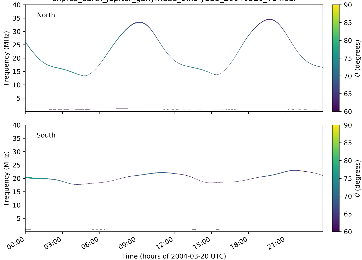
expres_earth_jupiter_ganymede_txka-y235_20040320_v14.cdf
