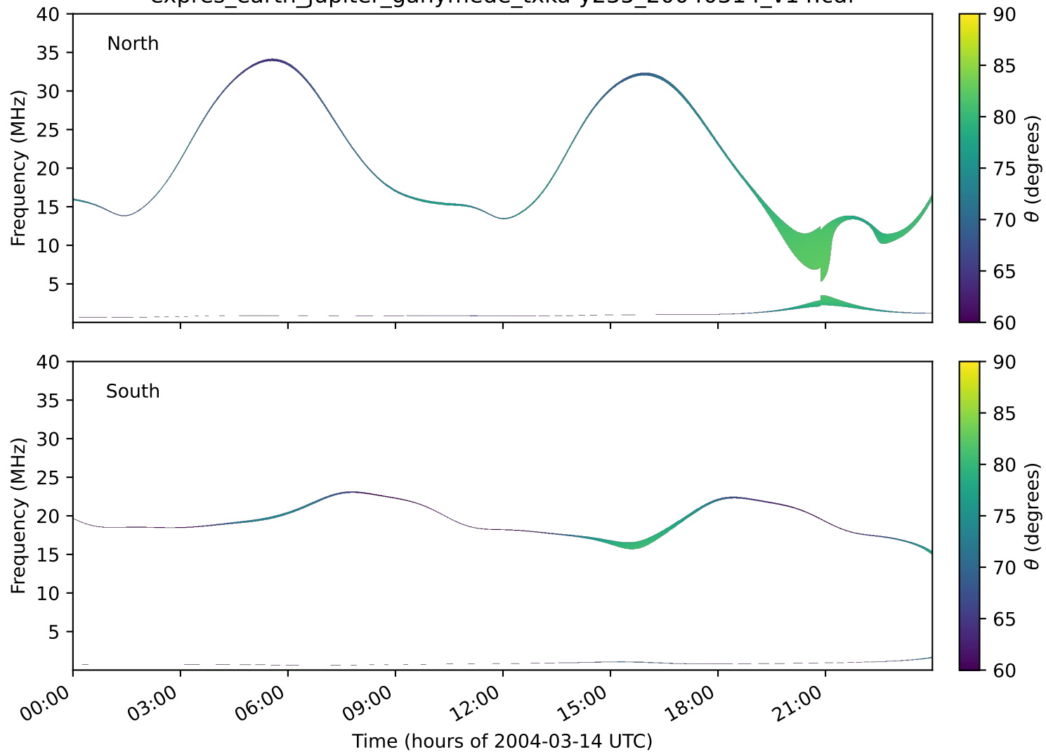
expres_earth_jupiter_ganymede_txka-y235_20040314_v14.cdf
