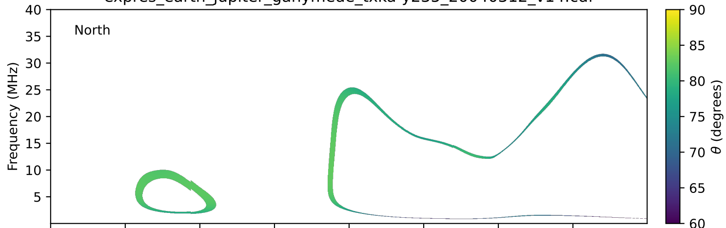
expres_earth_jupiter_ganymede_txka-y235_20040312_v14.cdf
